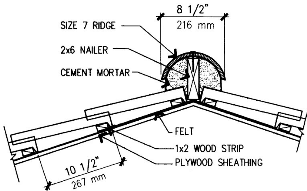
RIDGE DETAIL
